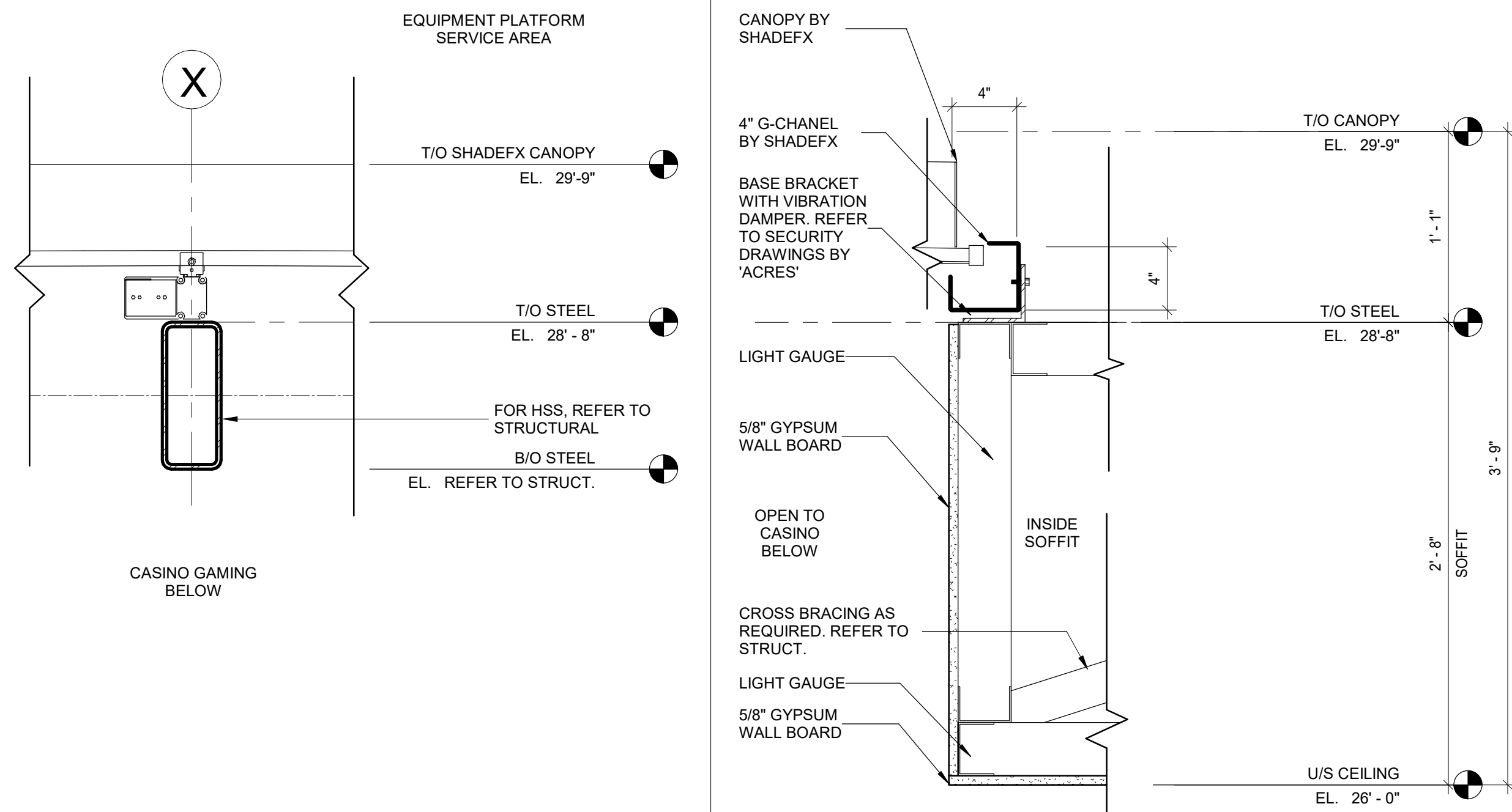
5 A-706 DETAIL - SECTION - RETRACTABLE CANOPY AT EQUIPMENT PLATFORM
