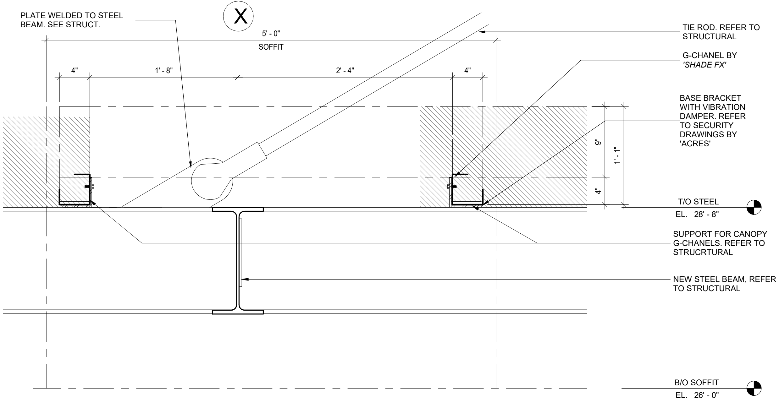
6 A-706 DETAIL SECTION - SHADEFX AT TIE ROD
