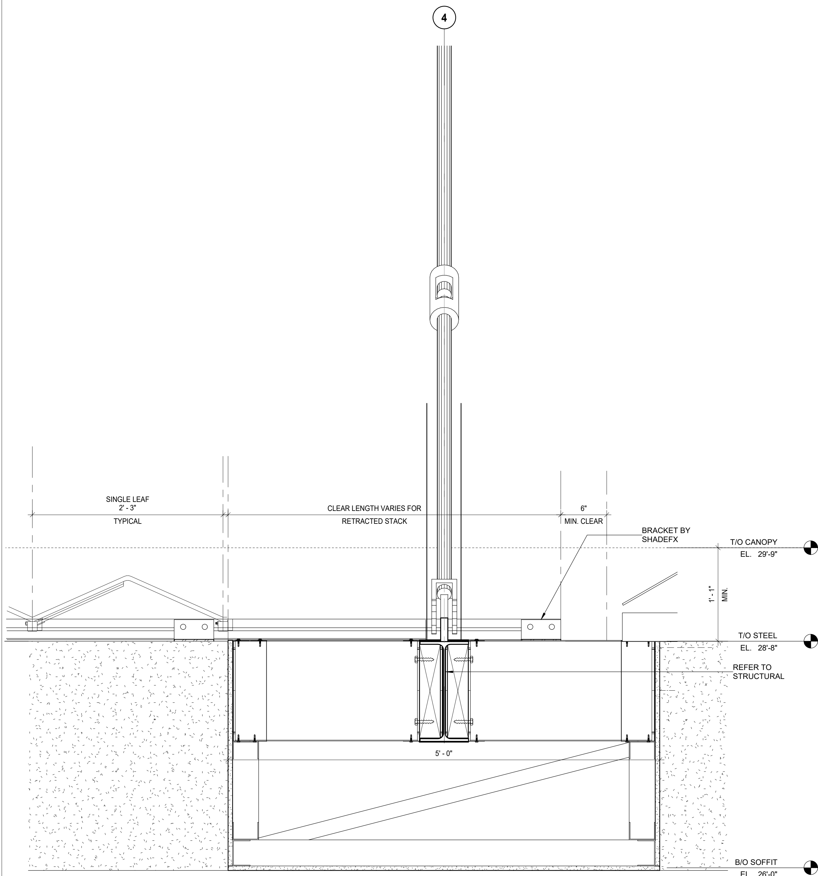
8 A-706 DETAIL - SECTION - RETRACTABLE CANOPY AT EQUIPMENT PLATFORM
