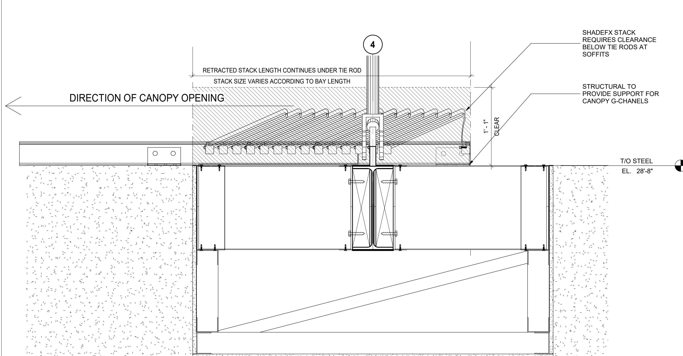
5 A-706 DETAIL - SECTION - RETRACTABLE CANOPY AT EQUIPMENT PLATFORM
