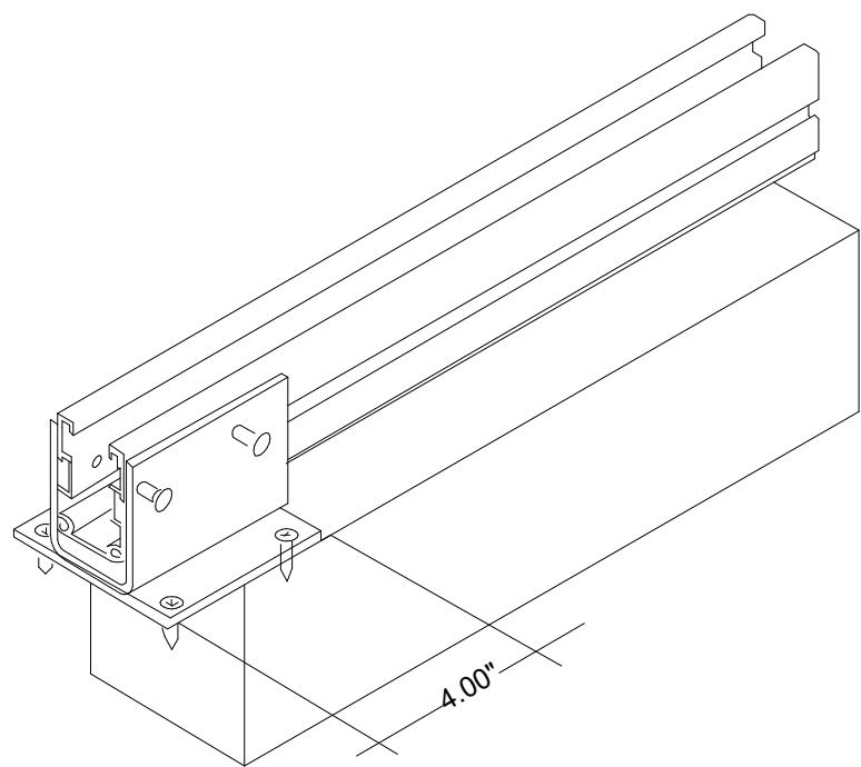
4 A-706 DETAIL - ISOMETRIC - VIBRATION COTROL
